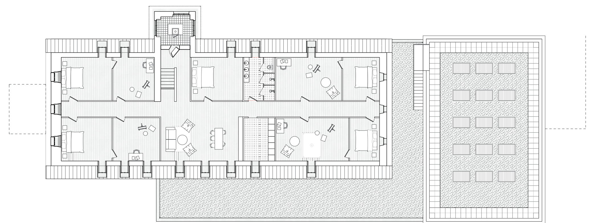
Plan combles
