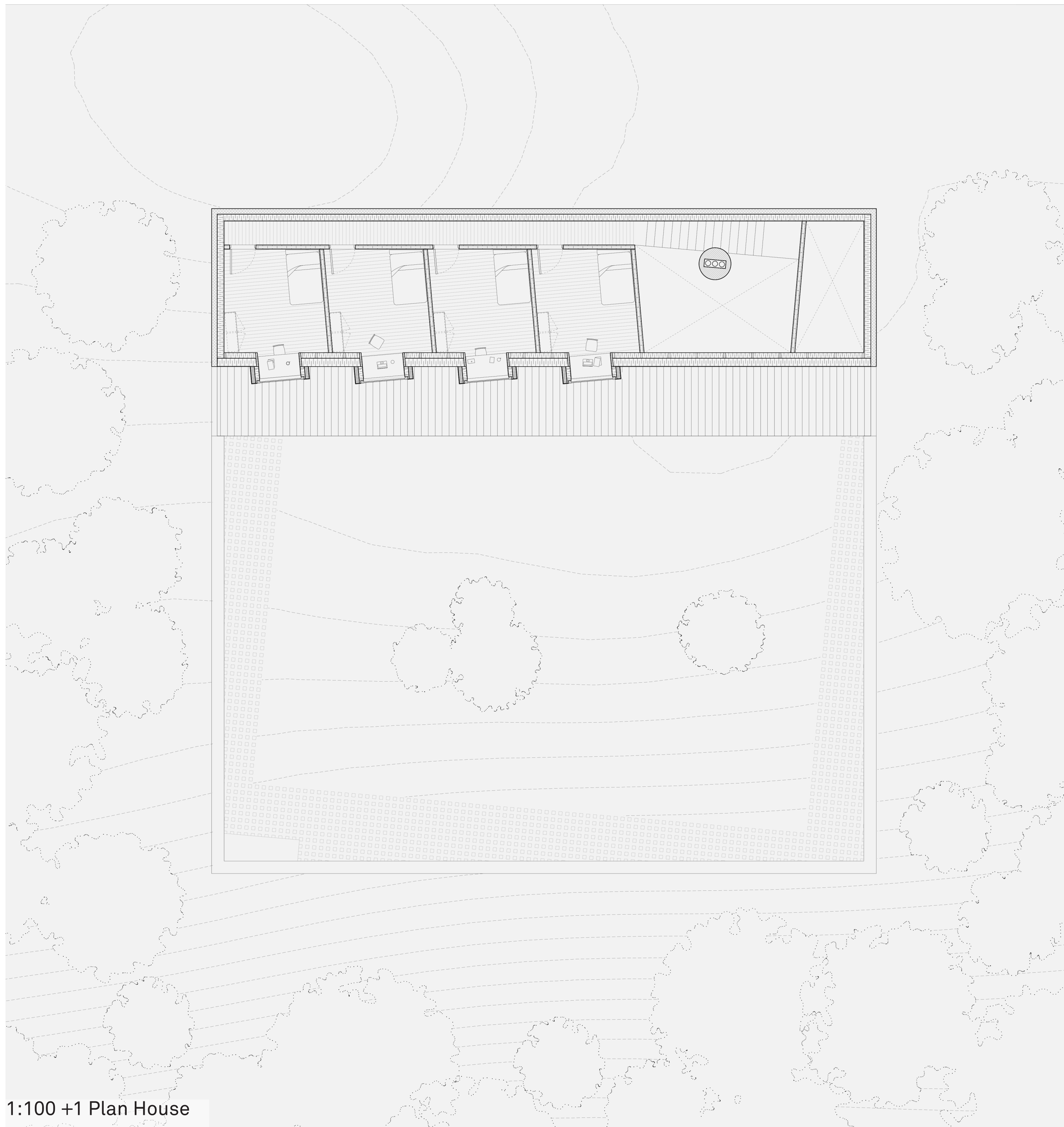
1:100 +1 Plan House
