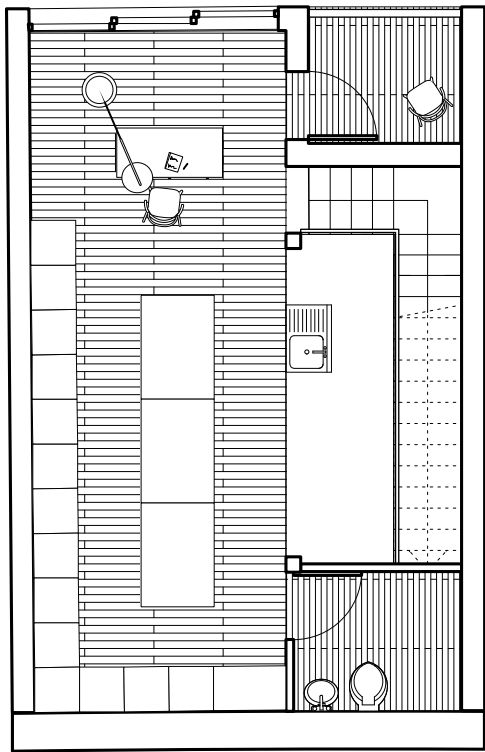
plan typ0 R-1 1:100
