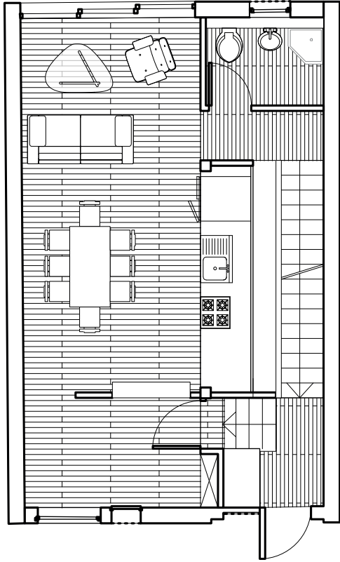
plan typ0 R0 1:100
