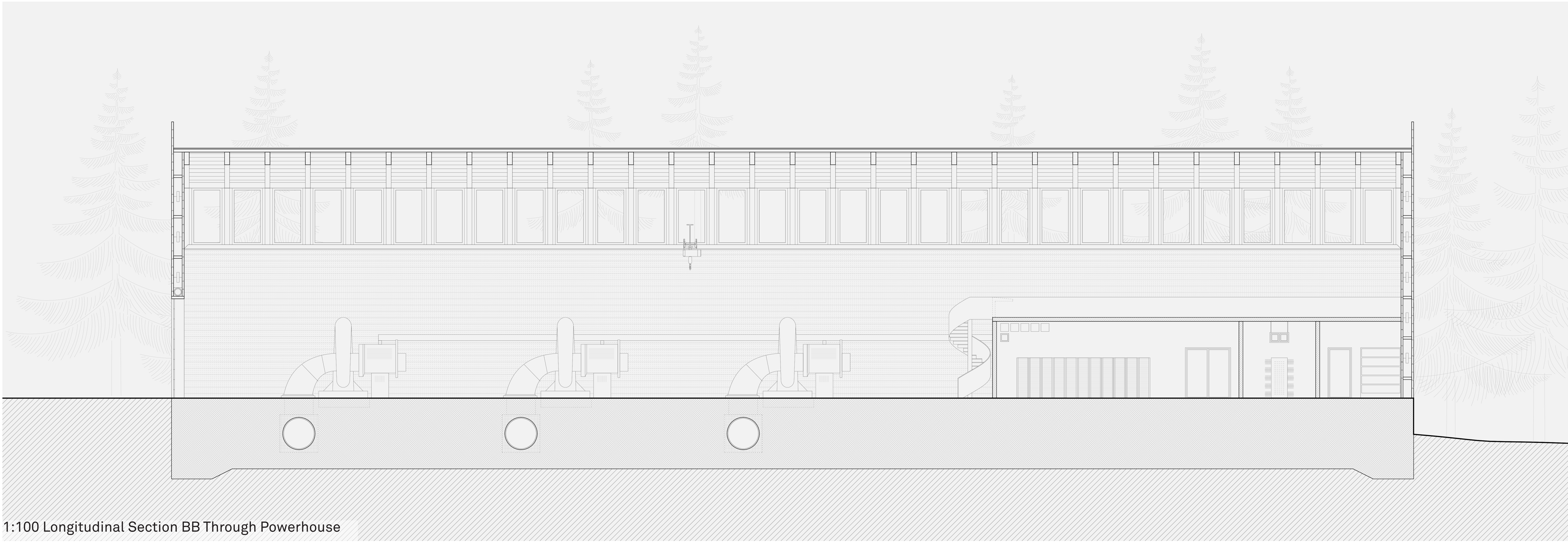
1:100 Longitudinal Section BB Through Powerhouse
