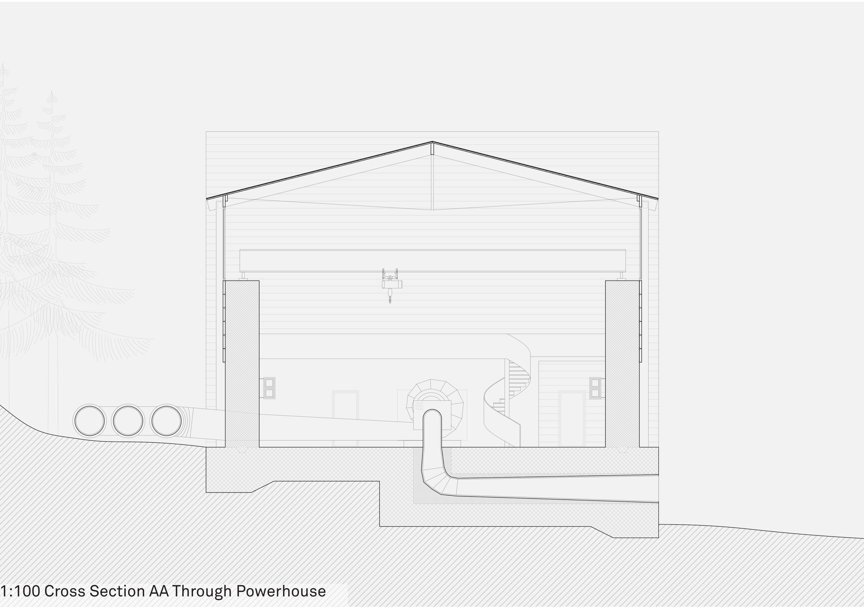
1:100 Cross Section AA Through Powerhouse
